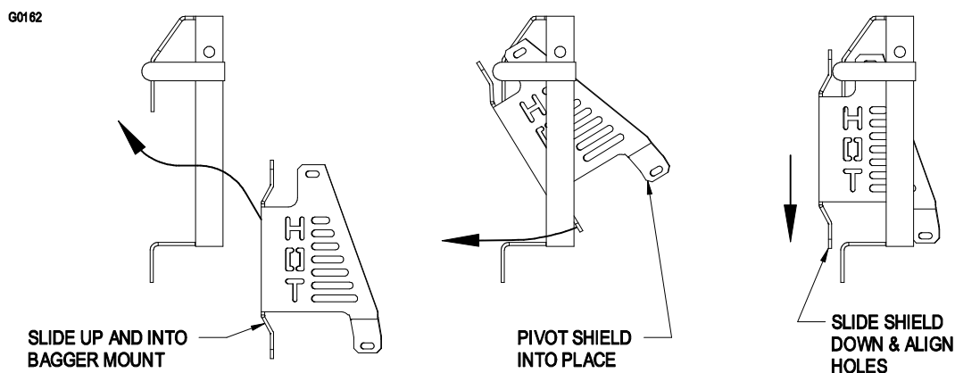
FIGURE 9 HOT ENGINE GUARD INSTALLATION
