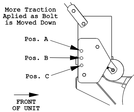
FIGURE 15 DRIVE BELT TENSION ADJUSTMENT POSITIONS
